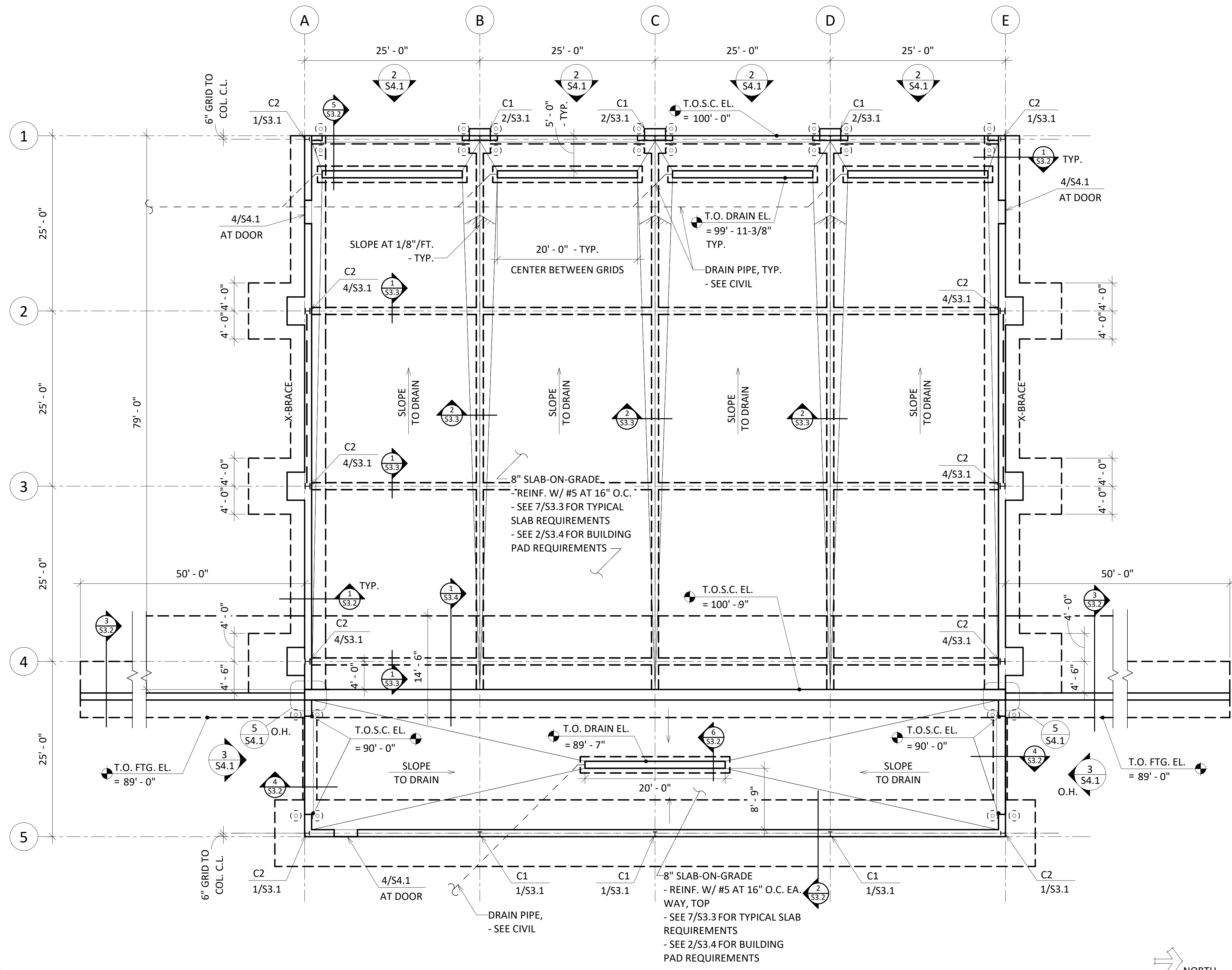
1 FOUNDATION PLAN 1/8" = 1'-0" 0 5 10 20
